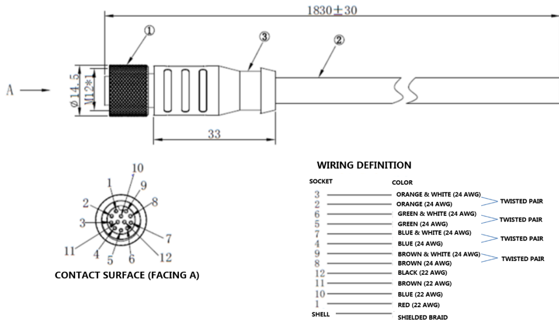
Figure 2.2 The 12-Pin Cable
