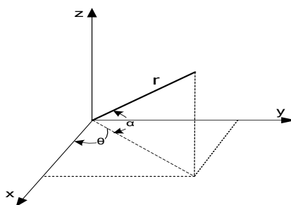
Figure 7.2 Coordinate Mapping
