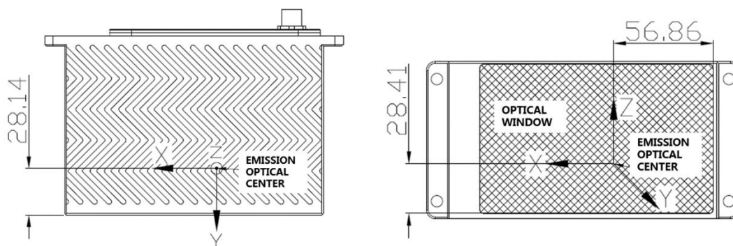
Figure 1.4 Optical Center of the CH64 Lidar
