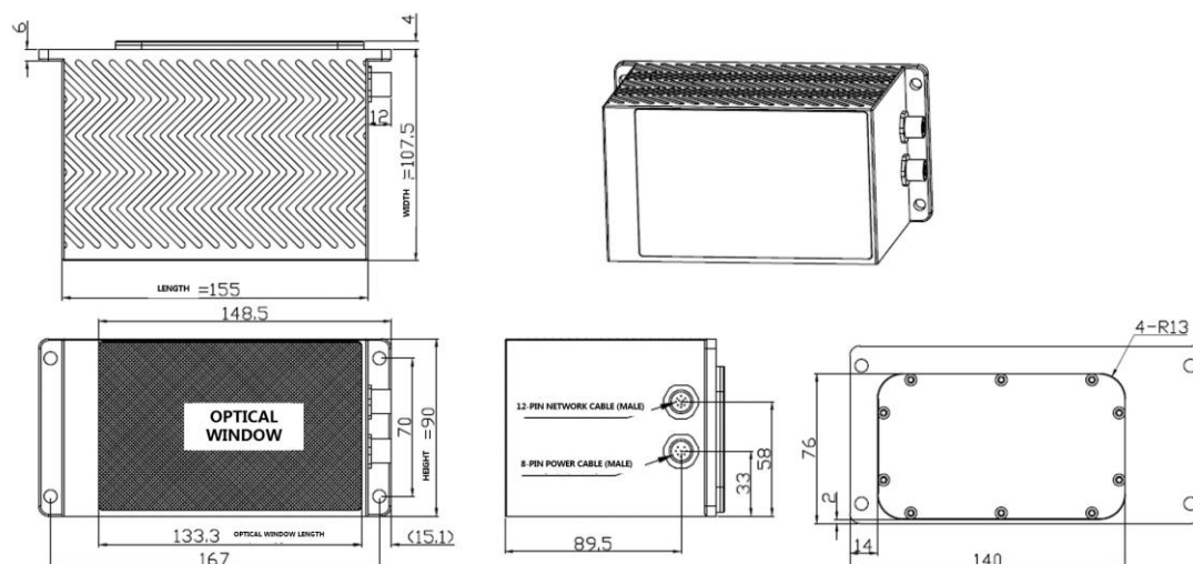
Figure 1.3 CH64 Lidar Dimensions (Cable Interface on the Side)
