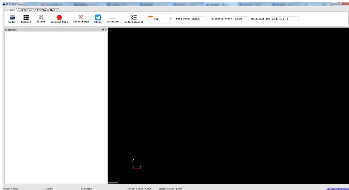
Figure 4.2 Initial Interface
