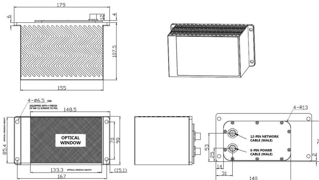
Figure 1.2 CH64 Lidar Dimensions (Cable Interface on the Back)
